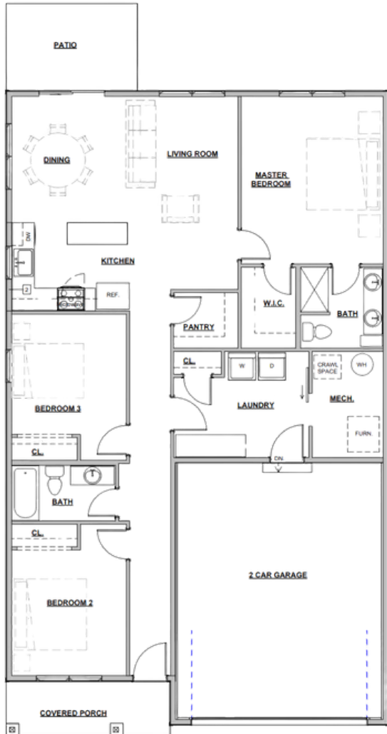
② FIRST FLOOR PLAN 1/4" = 1'-0"
